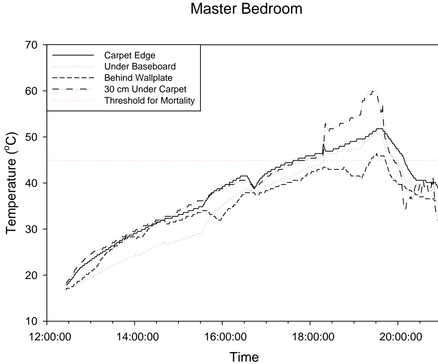
Figure 4.4. Heat up profile for the master bedroom in a house receiving a heat treatment to control bed bugs.
