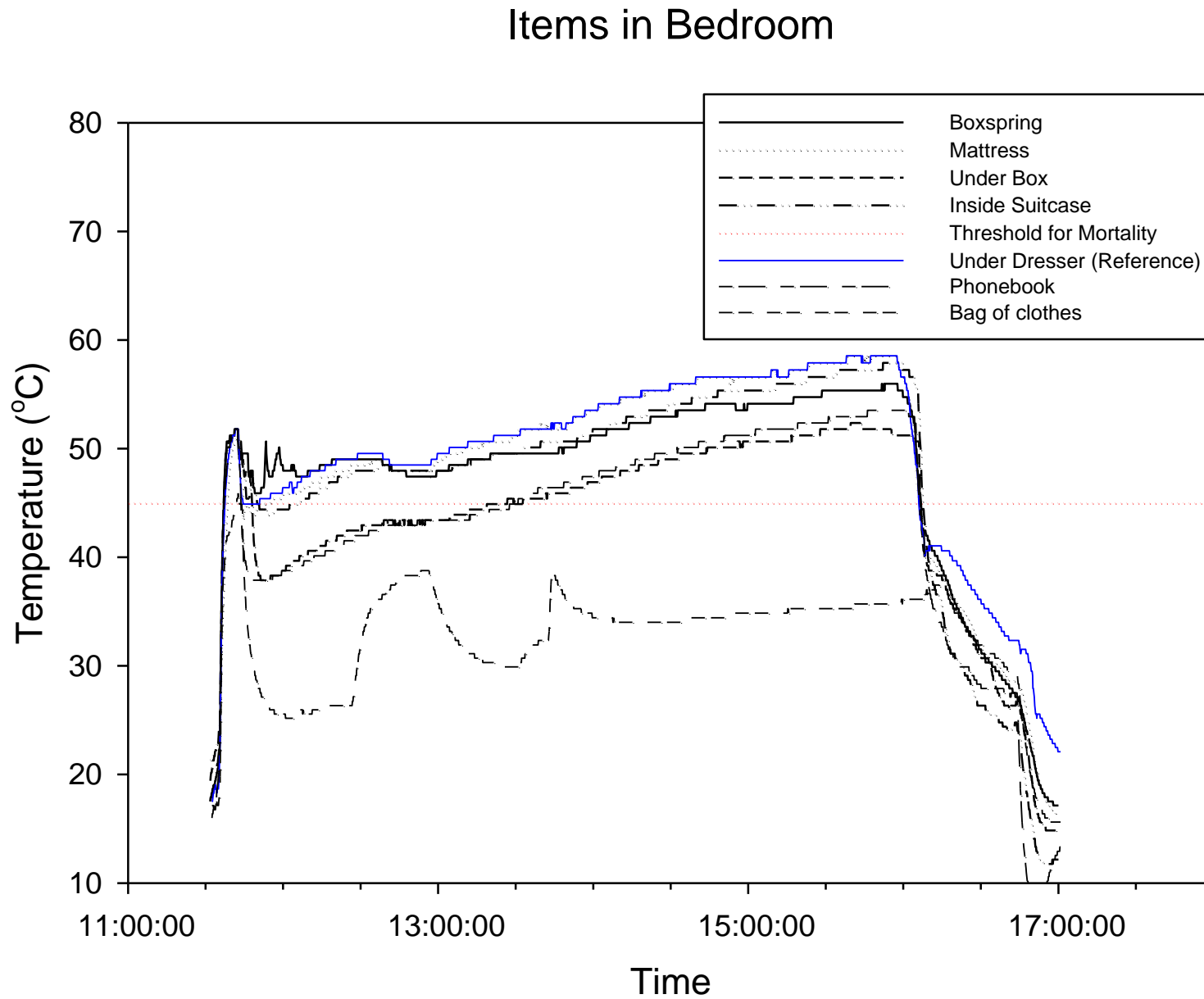
Figure 4.2. Heat up profile for different articles an apartment bedroom. The reference temperature (blue line) represents measurement of the room temperature.
